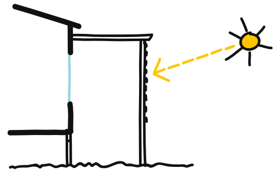
Figure 12 An example of an east or west-facing pergola with a vertical screen to block low-angle sun.
